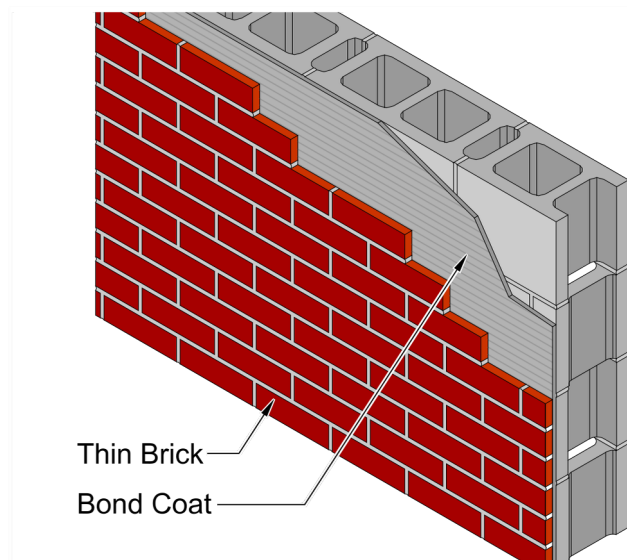
Figure 2 Thin Set Application on CMU
