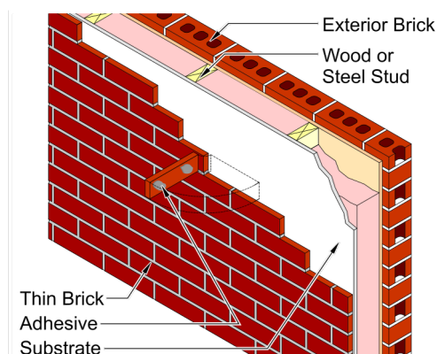
Figure 10 Interior Thin Set Application on Studs
