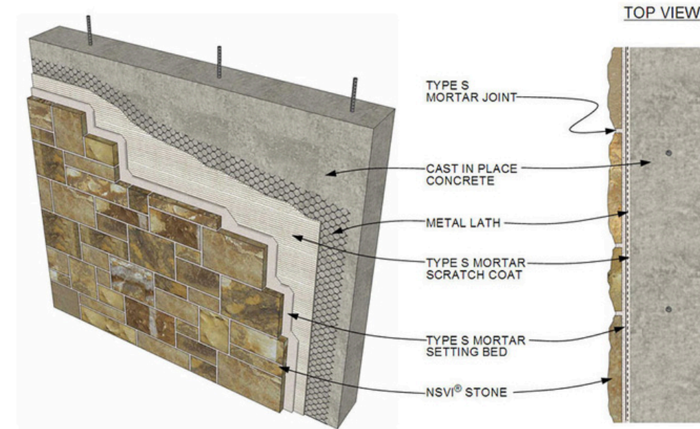
STONE VENEER ON CAST IN PLACE CONCRETE
