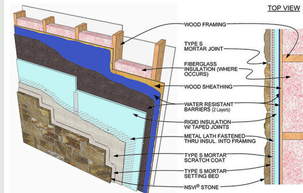
HIGH-R WALL WOOD FRAMING, RIGID INSULATION
