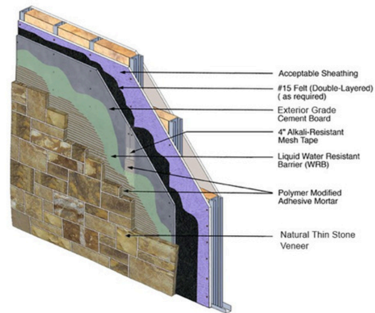
STONE VENEER ON CEMENT BOARD (Wood or Steel Studs)
