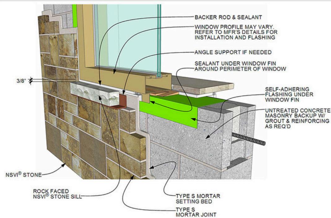
WINDOW SILL CONCRETE MASONRY BACKUP
