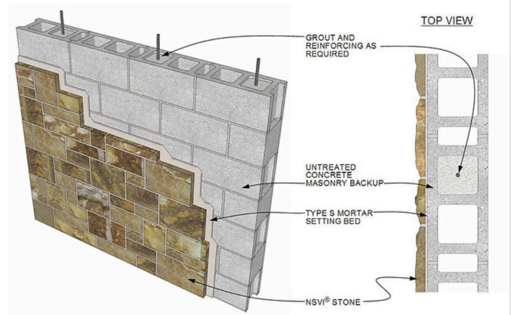
STONE VENEER ON CONCRETE MASONRY
