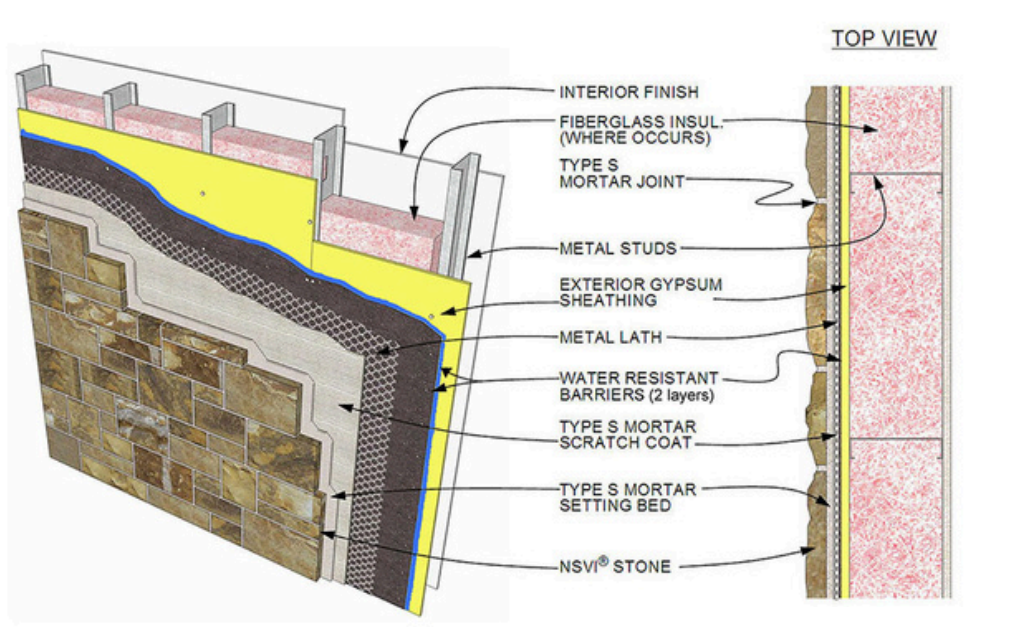
STONE VENEER ON METAL STUDS ON GYP. SHEATHING
