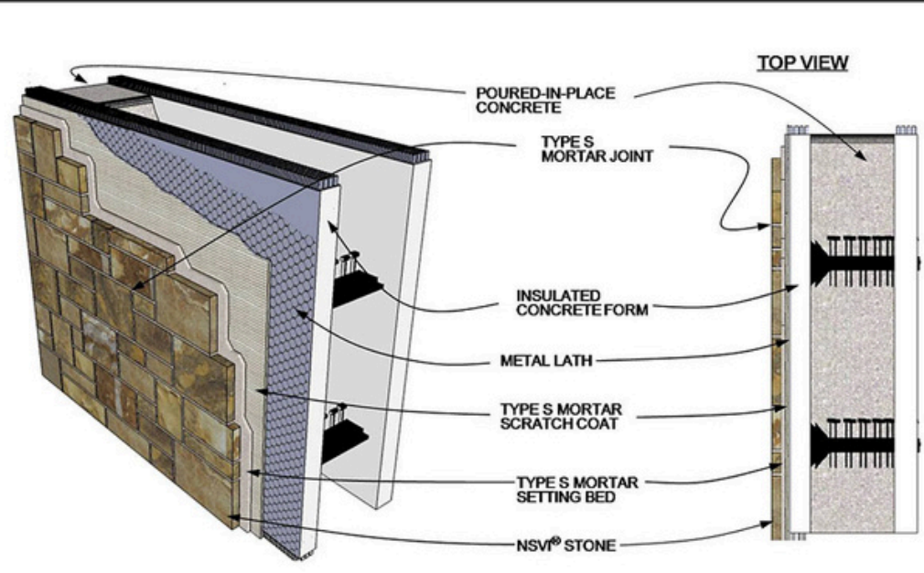
STONE VENEER ON INSULATED CONCRETE FORM
