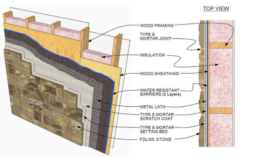
STONE VENEER ON WOOD FRAMING
